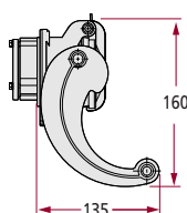
Embase semi-encastrée Semi-recessed socket
