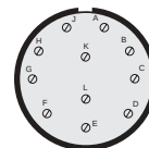
Disposition 18-11 11 contacts taille/size 16
