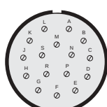
Disposition 20-16 16 contacts taille/size 16
