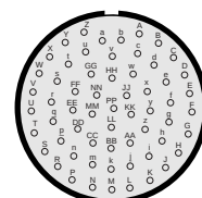
Disposition 24-61 61 contacts taille/size 20
