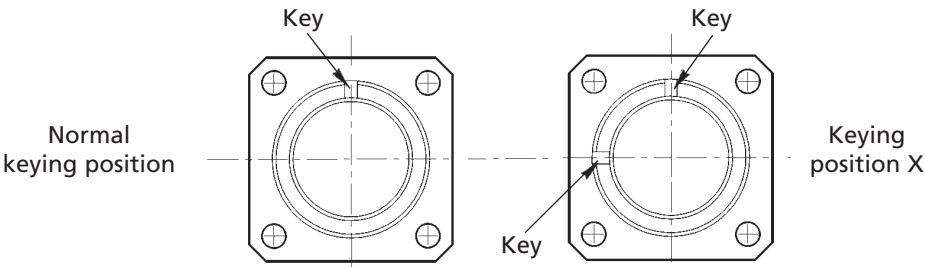
Receptacle front view
