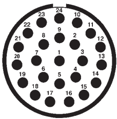
Arrangement 37-2 24 contacts size 16 Service 1
