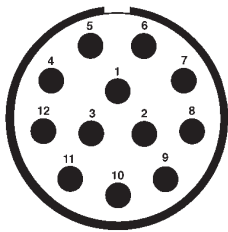
Arrangement 37-3 12 contacts size 12 Service 1
