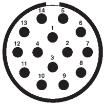
Arrangement 27-2 14 contacts size 16 Service 2
